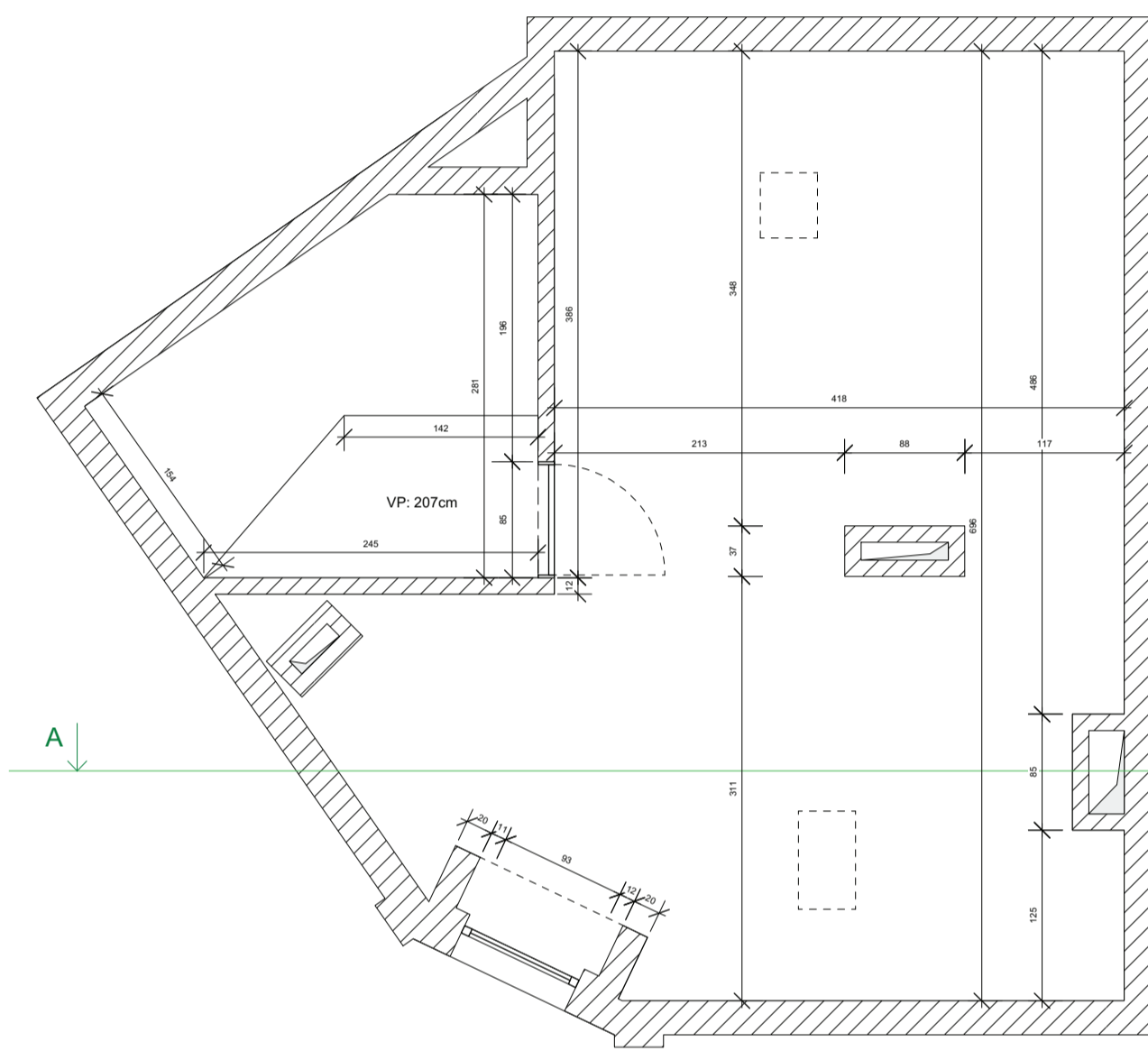
ZOLDER
